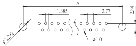
FEMALE/MALE
