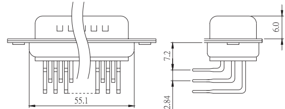
50 POSITION MALE
