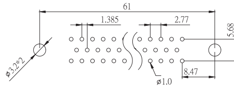
50 POSITION FEMALE/MALE
