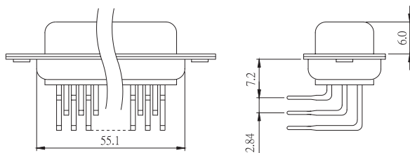
50 POSITION FEMALE
