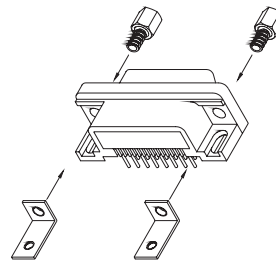
W/NON-THREAD L-SHAPE SCREW FIXED
