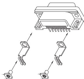
RIVET W/BOARDLOCK
