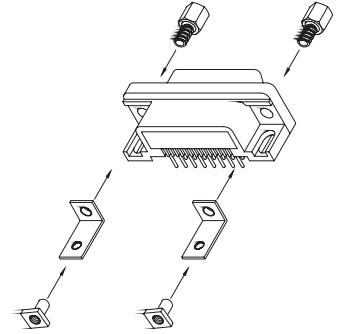
RIVET W/NON-THREAD L-SHAPE SCREW FIXED
