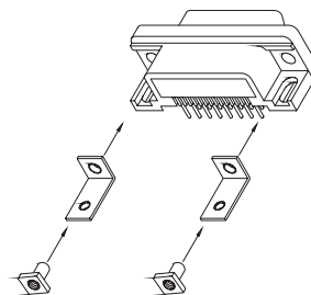
RIVET W/NON-THREAD L-SHAPE
